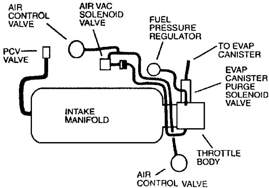
Fig. 21: Vacuum Diagram - 4.0L Aurora & 4.6L SFI (VIN Y & 9) DeVille, Eldorado & Seville Courtesy of General Motors Corp.
