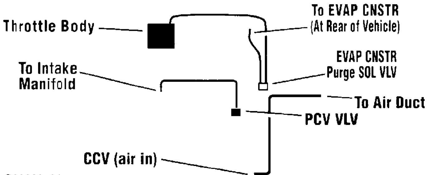
Fig. 4: Vacuum Diagram - 1.9L SFI (VIN 7) Saturn "S" Series (Federal) Courtesy of General Motors Corp.
