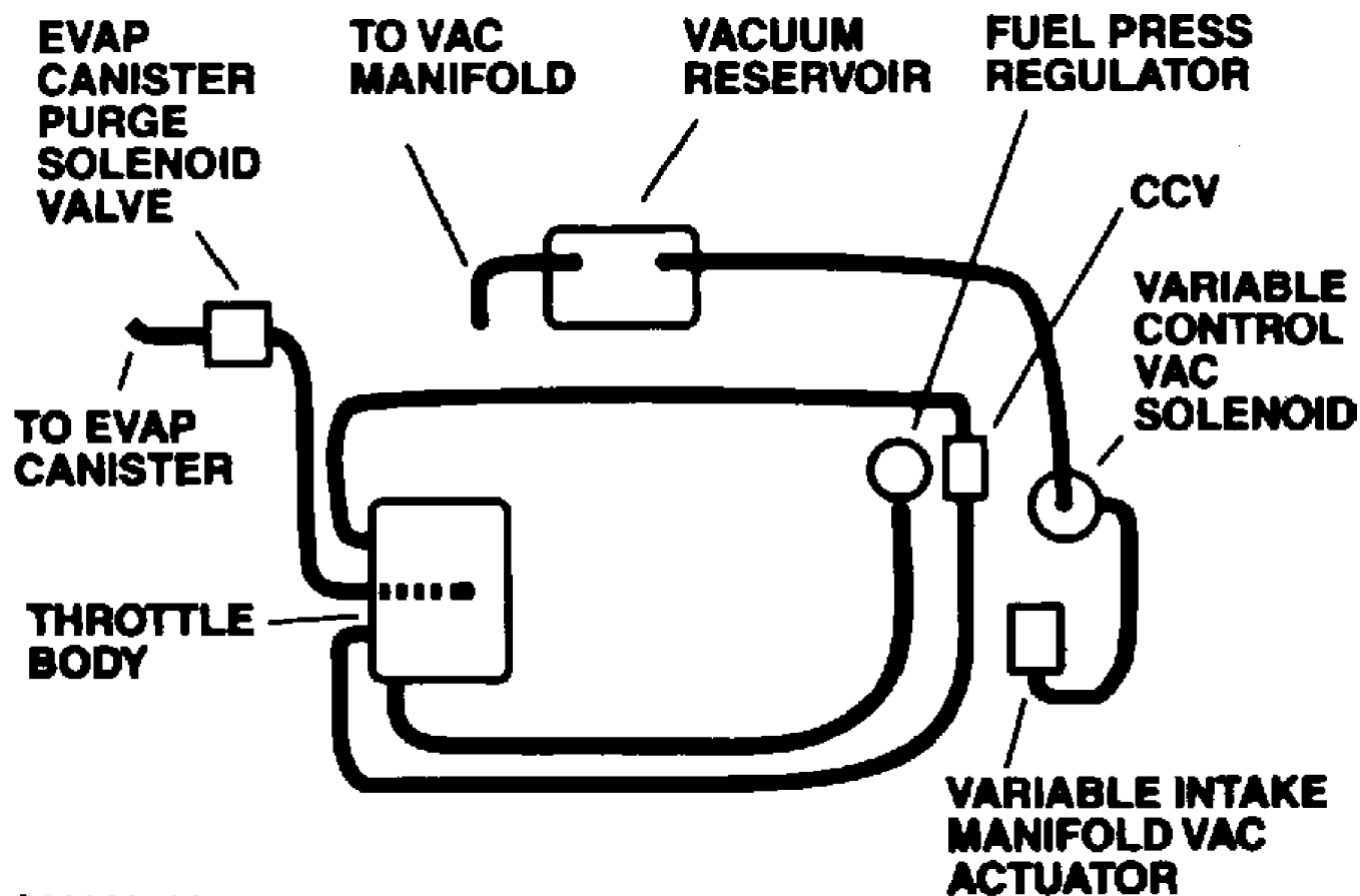
Fig. 12: Vacuum Diagram - 3.0L SFI (VIN R) Saturn "L" Series Courtesy of General Motors Corp.
