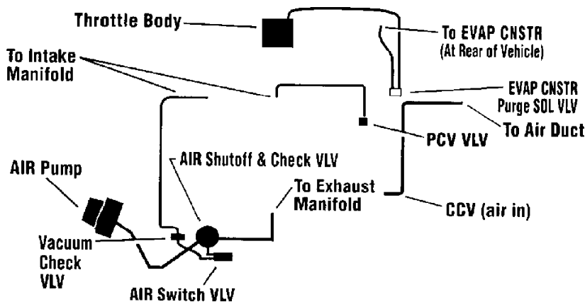
Fig. 3: Vacuum Diagram - 1.9L SFI (VIN 7) Saturn "S" Series (California) Courtesy of General Motors Corp.
