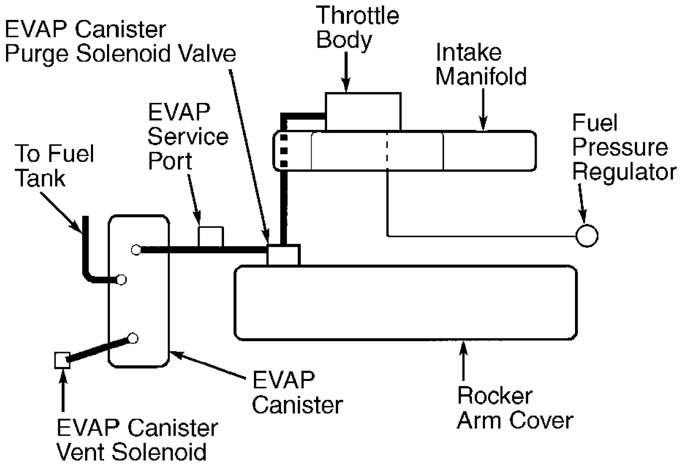
Fig. 7: Vacuum Diagram - 2.2L SFI (VIN 4) Cavalier & Sunfire Courtesy of General Motors Corp.
