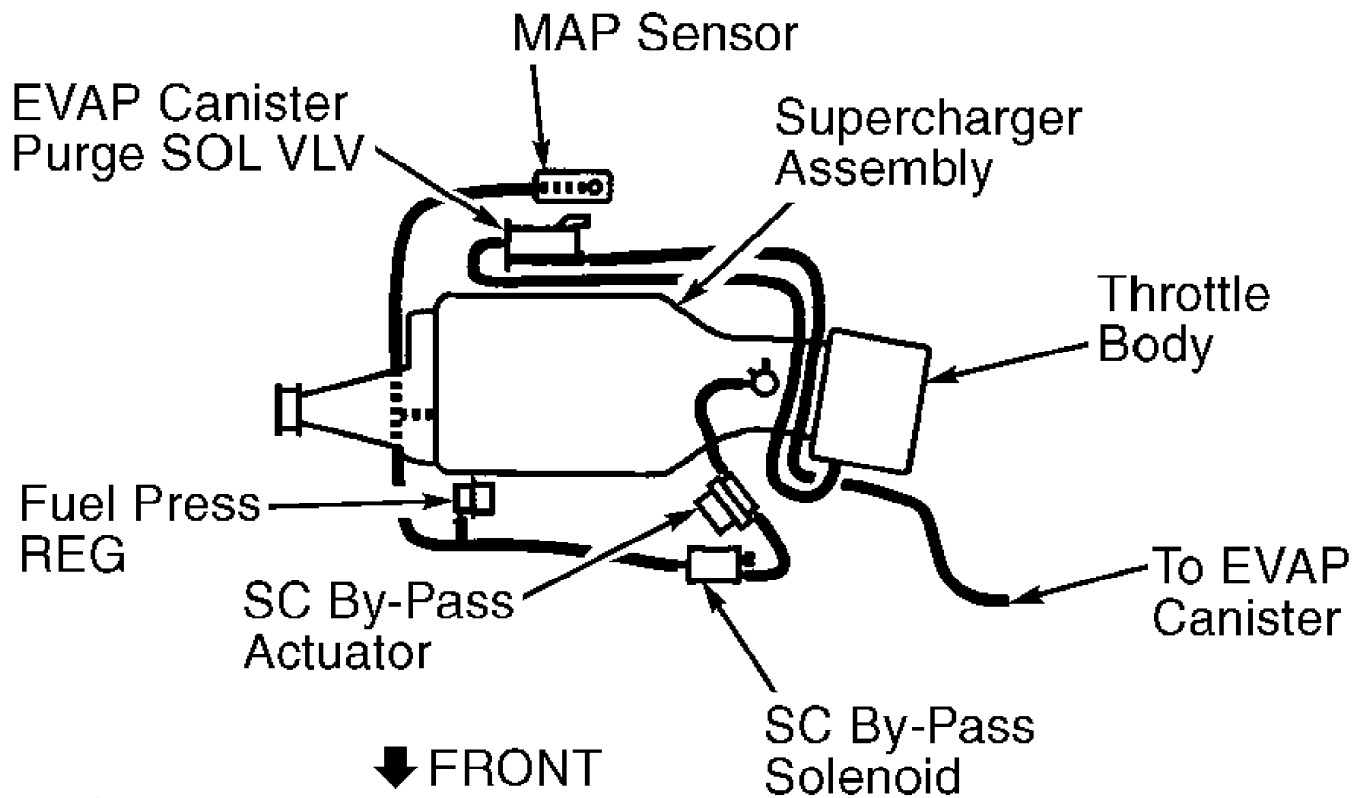
Fig. 20: Vacuum Diagram - 3.8L SFI (VIN 1) Bonneville, Grand Prix, Park Avenue & Regal Courtesy of General Motors Corp.
