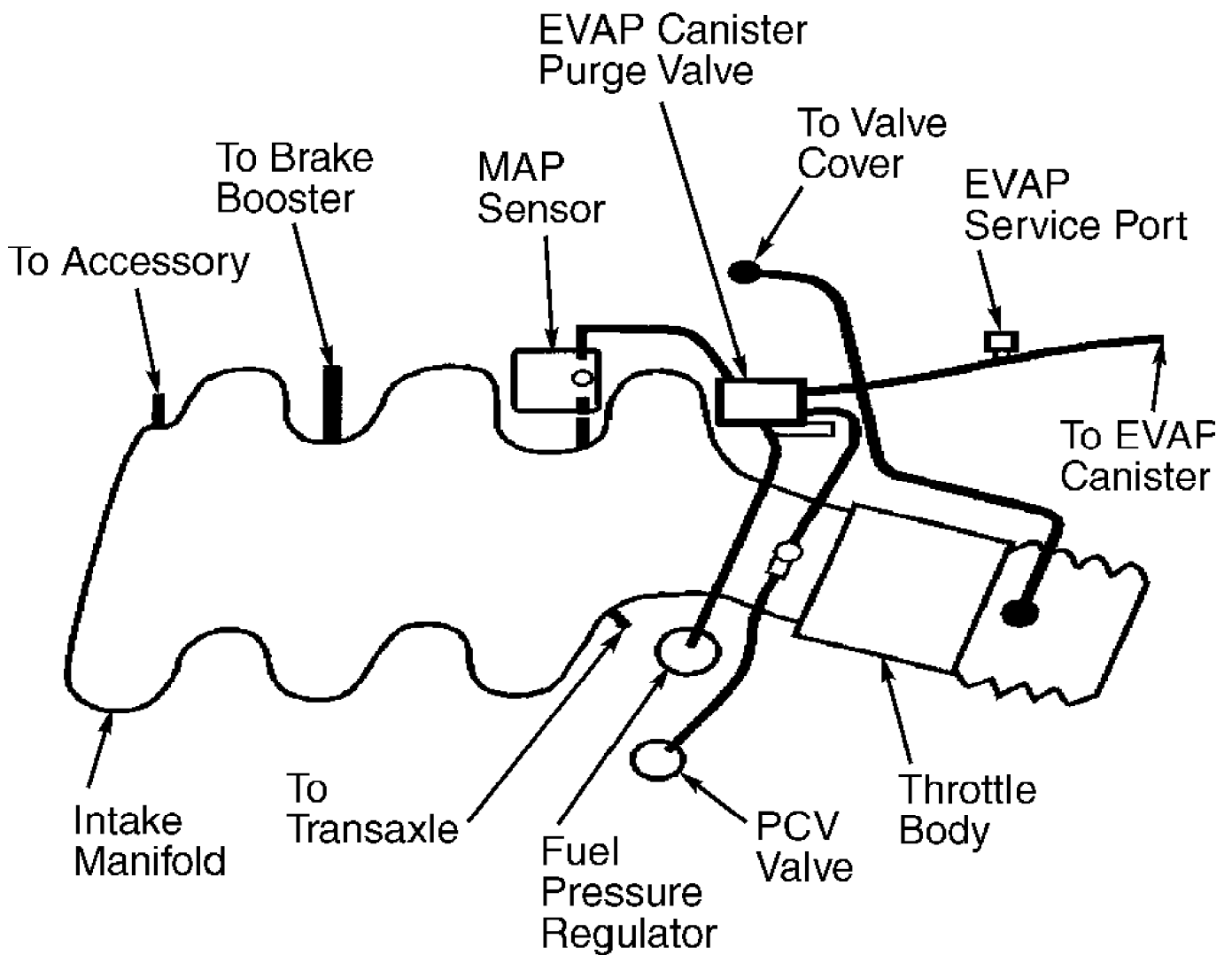
Fig. 14: Vacuum Diagram - 3.1L SFI (VIN J) Lumina Courtesy of General Motors Corp.
