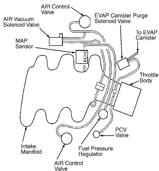
Fig. 13: Vacuum Diagram - 3.1L SFI (VIN J) Century, Grand Prix & Malibu, & 3.4L SFI (VIN E) Impala & Monte Carlo Courtesy of General Motors Corp.
