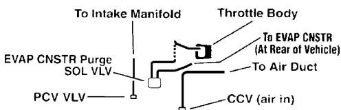
Fig. 6: Vacuum Diagram - 1.9L SFI (VIN 8) Saturn "S" Series (Federal) Courtesy of General Motors Corp.
