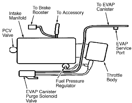
Fig. 19: Vacuum Diagram - 3.8L SFI (VIN K) Impala Courtesy of General Motors Corp.
