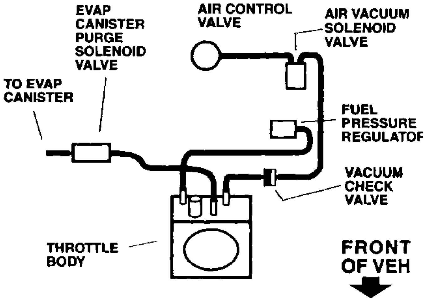
Fig. 9: Vacuum Diagram - 2.2L SFI (VIN F) Saturn "L" Series (California Emissions) Courtesy of General Motors Corp.
