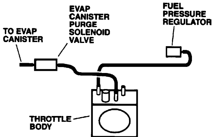
Fig. 8: Vacuum Diagram - 2.2L SFI (VIN F) Saturn "L" Series (Except California Emissions) Courtesy of General Motors Corp.
