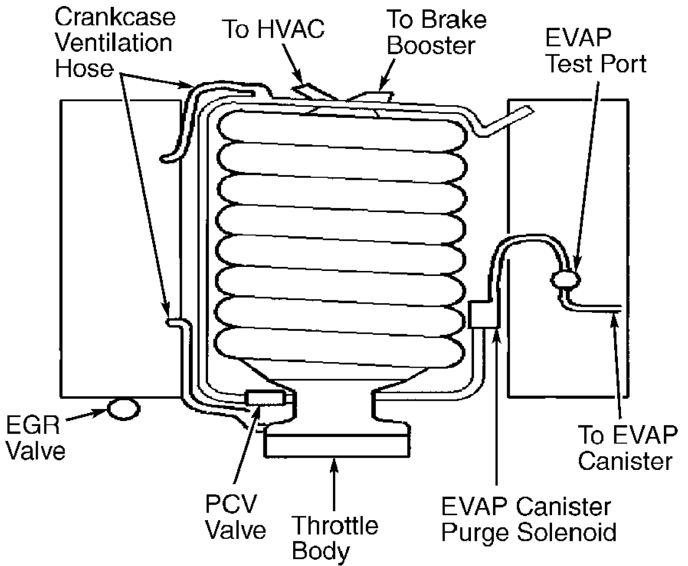
Fig. 22: Vacuum Diagram - 5.7L SFI (VIN G) Camaro, Corvette & Firebird Courtesy of General Motors Corp.
