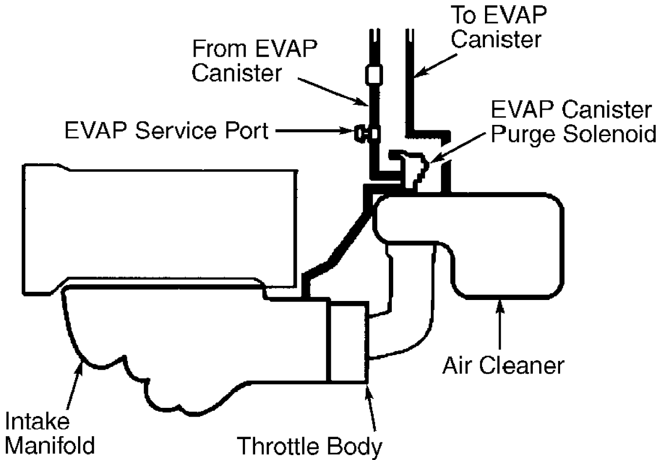
Fig. 2: Vacuum Diagram - 1.8L SFI (VIN 8) Prizm Courtesy of General Motors Corp.
