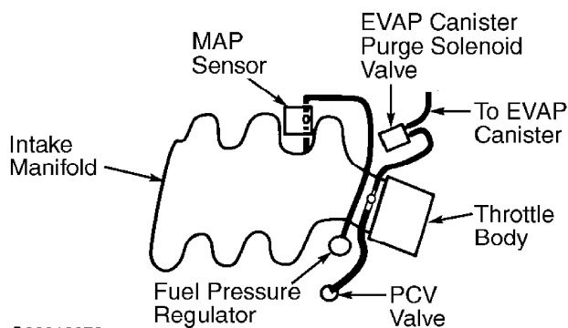
Fig. 15: Vacuum Diagram - 3.1L SFI (VIN J) Century, Grand Prix, Lumina & Malibu, & 3.4L SFI (VIN E) Alero, Grand Am, Impala & Monte Carlo (Federal) Courtesy of General Motors Corp.
