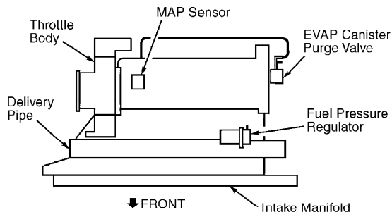
G98J00264 Fig. 1: Vacuum Diagram - 1.3L SFI (VIN 2) Metro Courtesy of General Motors Corp.
