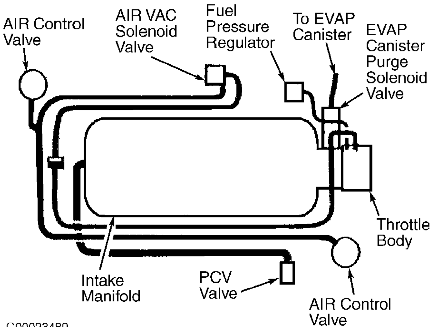
Fig. 16: Vacuum Diagram - 3.5L SFI (VIN H) Aurora & Intrigue Courtesy of General Motors Corp.
