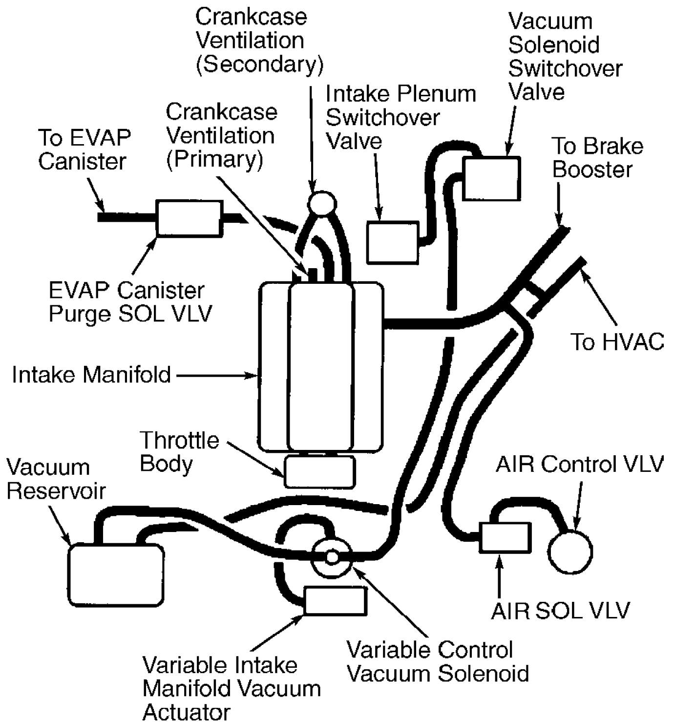
Fig. 11: Vacuum Diagram - 3.0L SFI (VIN R) Catera Courtesy of General Motors Corp.
