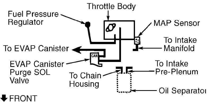
Fig. 10: Vacuum Diagram - 2.4L SFI (VIN T) Alero, Cavalier, Grand Am & Sunfire Courtesy of General Motors Corp.
