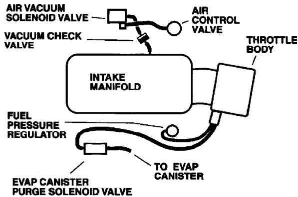
Fig. 17: Vacuum Diagram - 3.8L SFI (VIN K) Bonneville, Grand Prix, LeSabre, Park Avenue & Regal Courtesy of General Motors Corp.
