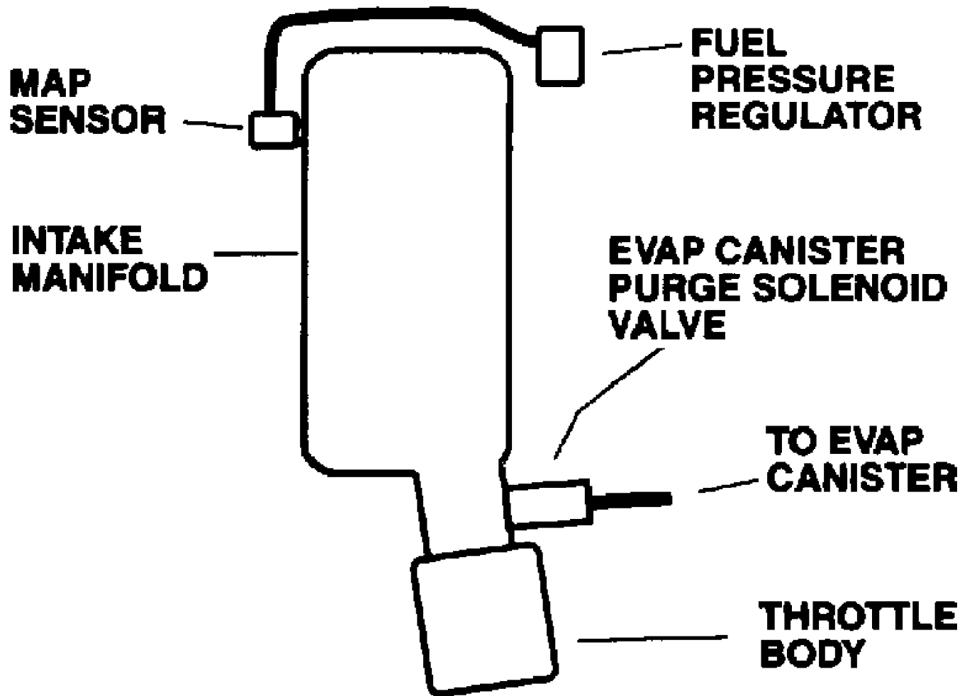
Fig. 18: Vacuum Diagram - 3.8L SFI (VIN K) Camaro & Firebird Courtesy of General Motors Corp.
