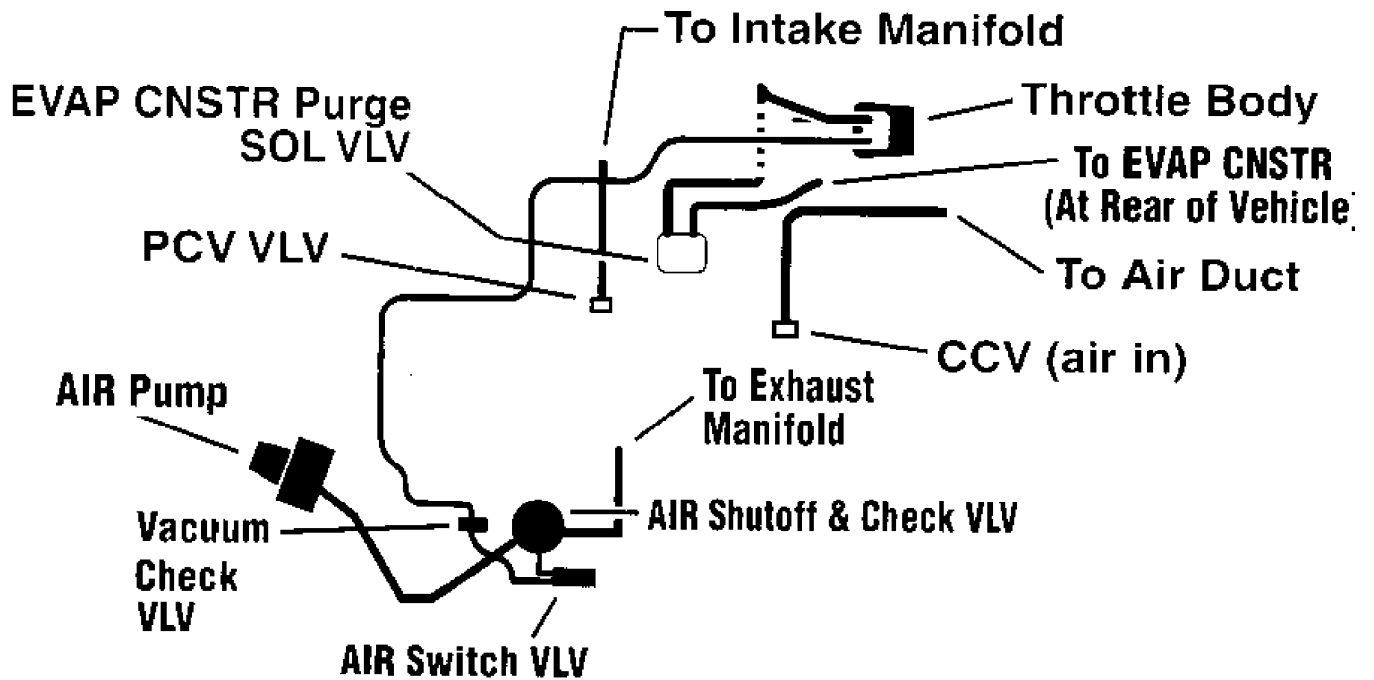
Fig. 4: Vacuum Diagram - 1.9L SFI (VIN 7) Saturn "S" Series (Federal) Courtesy of General Motors Corp.
